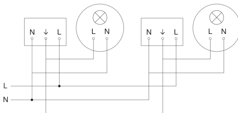
Master/slave interconnection circuit diagram
