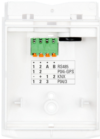
Fig. 14 Connect KNX data (+/-) and power supply (12...40V DC, 12...28V AC, 1/2) to the connector.
