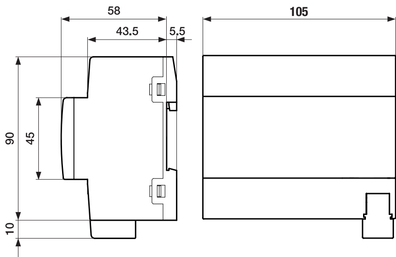
Dimension drawing
